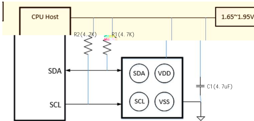
Figure 6. External Connection
